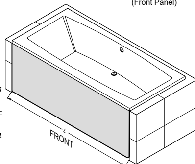
BETWEEN-WALLS APPLICATION (Front Panel)
